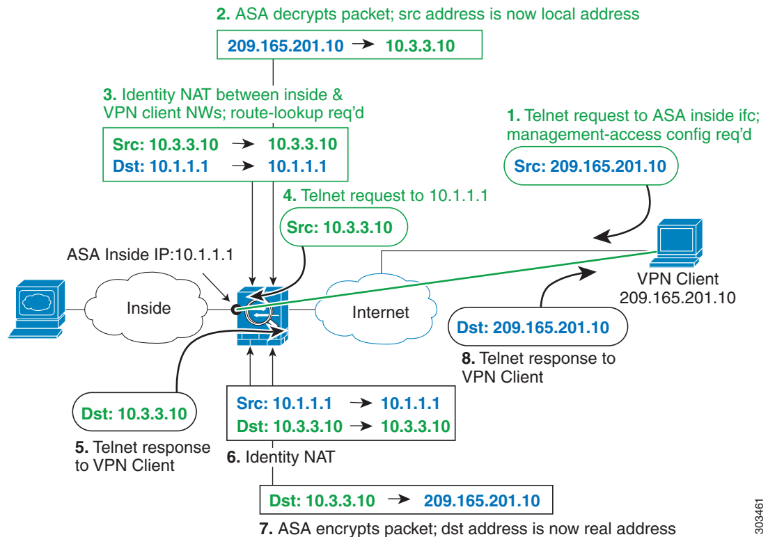
Figure 3-25 VPN Management Access
