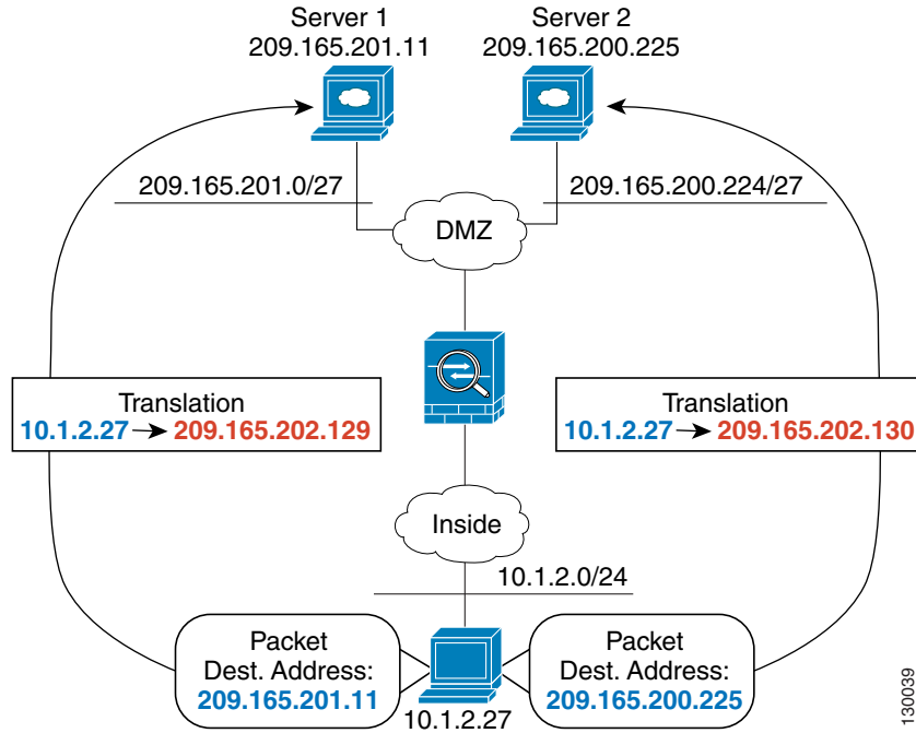
Figure 5-1 Twice NAT with Different Destination Addresses
