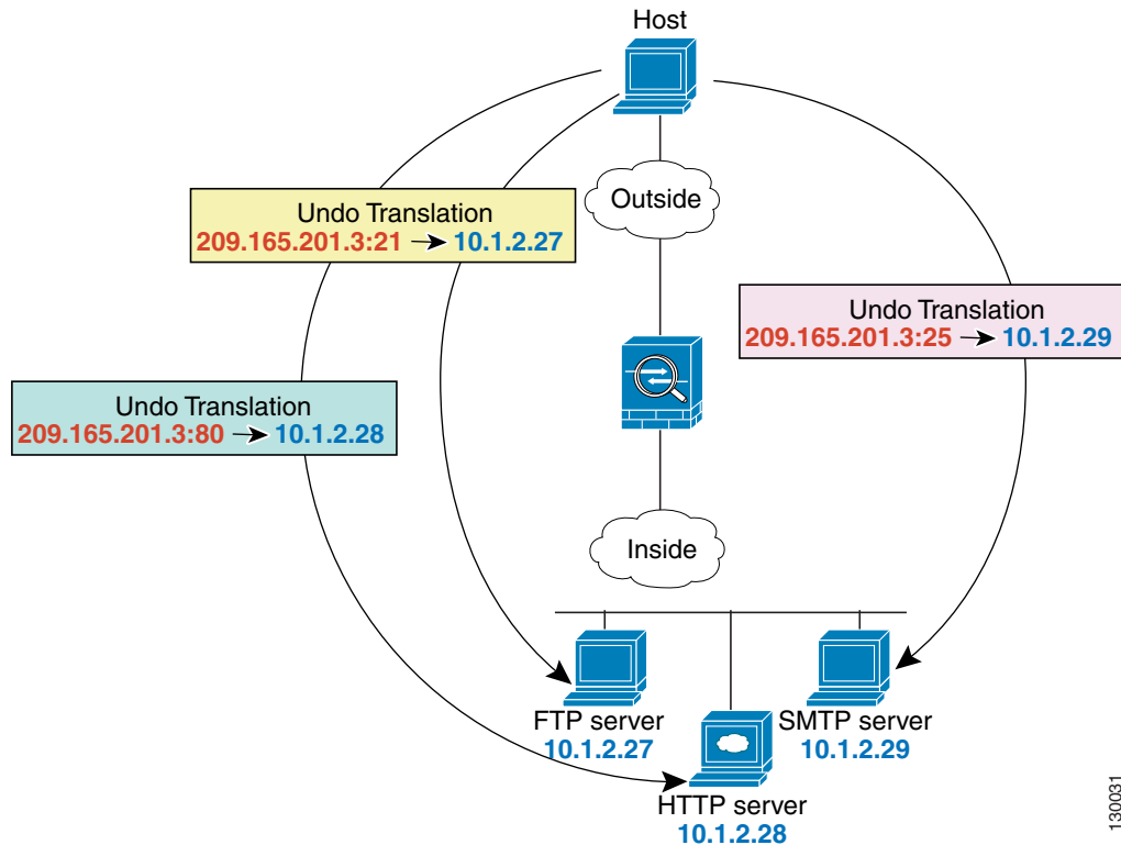
Figure 6-8 Static PAT
