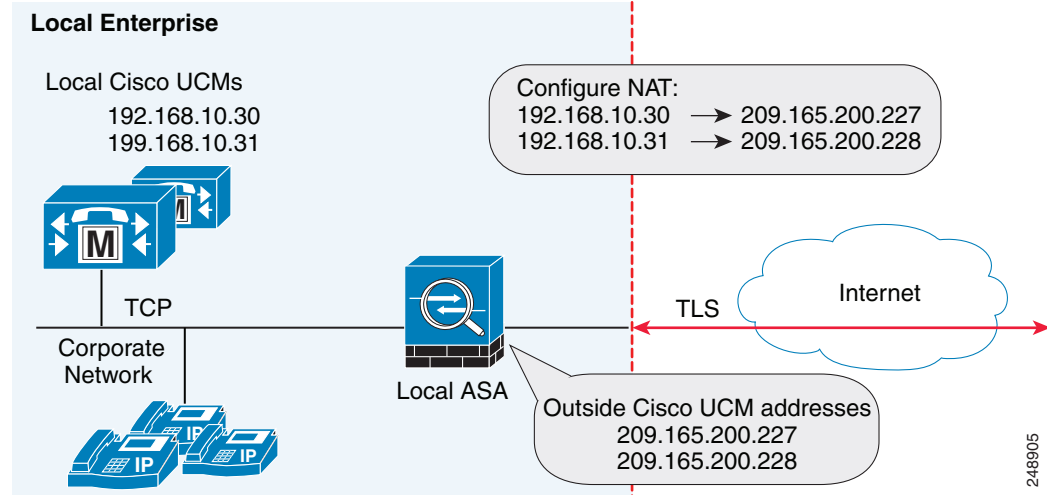
Figure 21-7 Example for Configuring NAT for a Deployment
