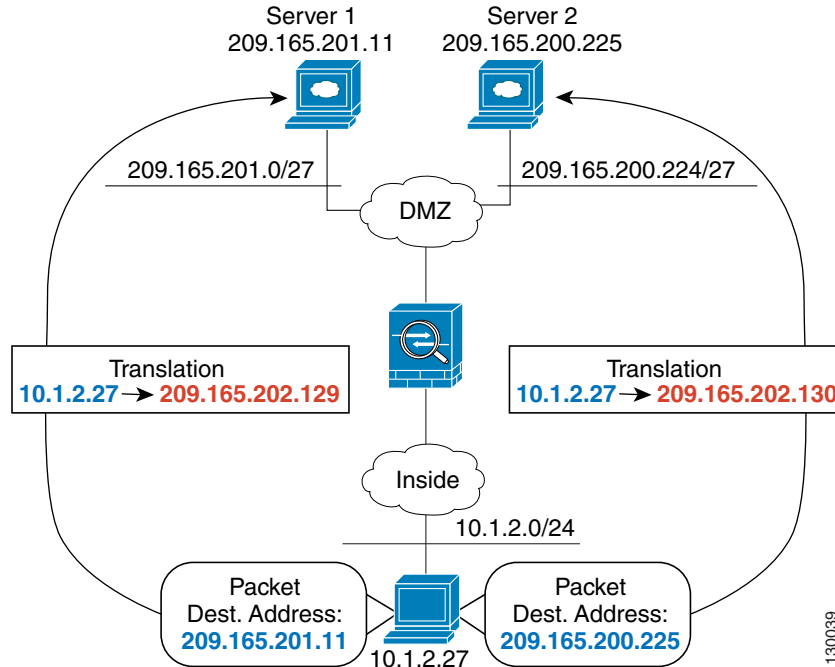
Figure 6-9 Policy NAT with Different Destination Addresses
